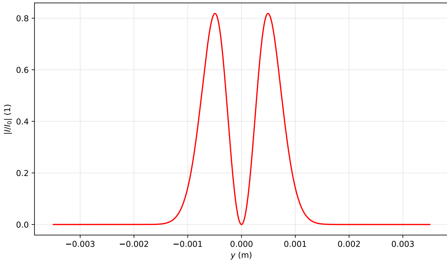
Intensity profile I(x=0, y, z=0.080)/I_0 , P_{in}=9.0P_{cr} , artificial time
